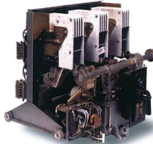
ITE KD circuit breaker before refurbishment
