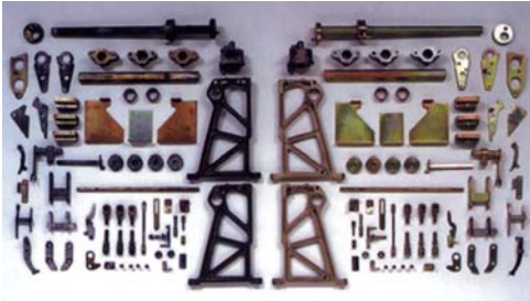
Mechanism parts from an ITE KD circuit breaker before and after refurbishment
