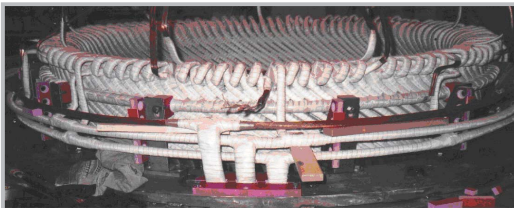
One of six motor rewinds completed for Virginia Power (Westinghouse, 6000 HP, 4160 V)
